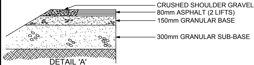
DETAIL 'A' → ACCESS ROUTE SERVING 3-5 UNITS STRATA : LEVEL 2
