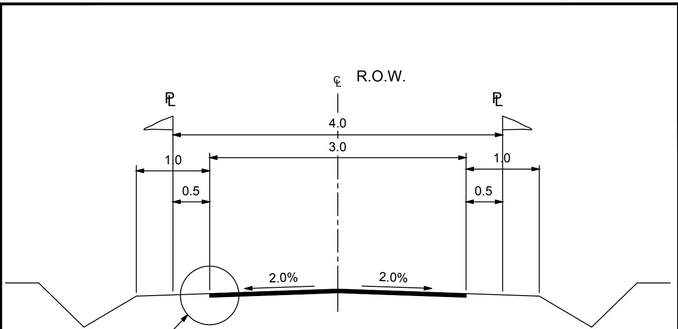
DETAIL 'A' → ACCESS ROUTE SERVING 1-2 UNITS STRATA : LEVEL 1
